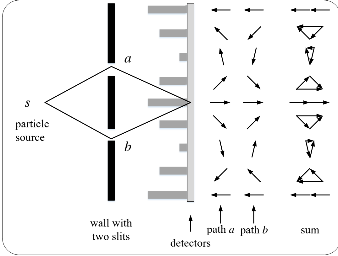
Figure 3: Schematic illustration of the double-slit experiment. The arrows represent the complex amplitudes for each path and their sum. Squaring the magnitude of the sum determines the corresponding probability. This leads to destructive and constructive interference, as displayed on the wall of detectors.
